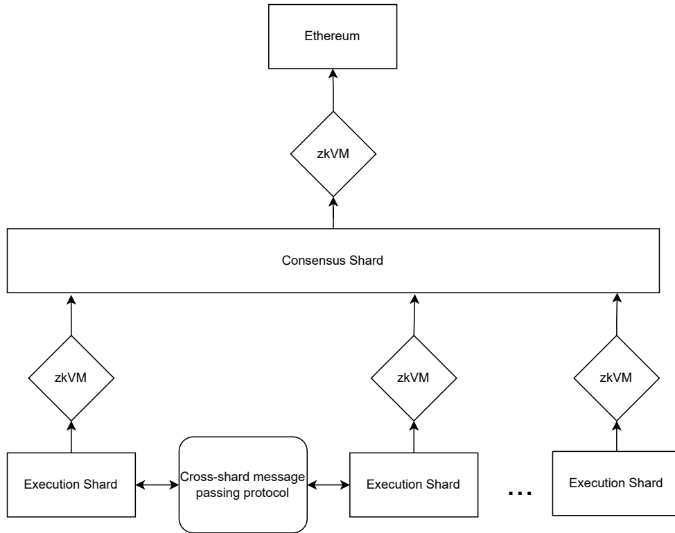
Figure 1: zkSharding Architecture
